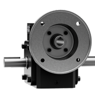
Flange Input Shaft Output Double End Output
